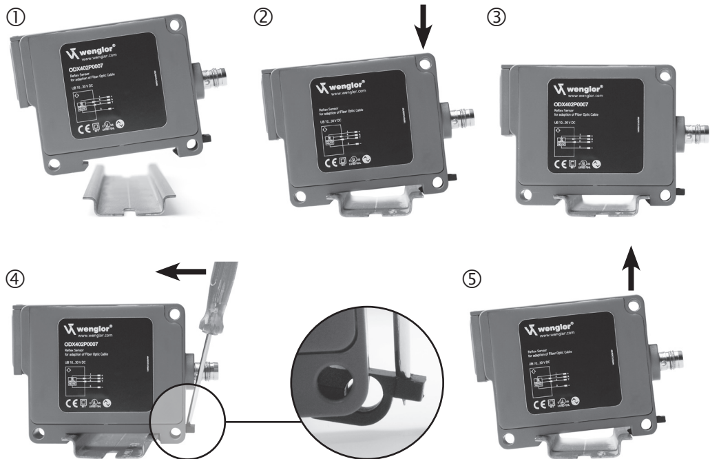
fig.1 Mounting of the Sensor to a DIN rail
