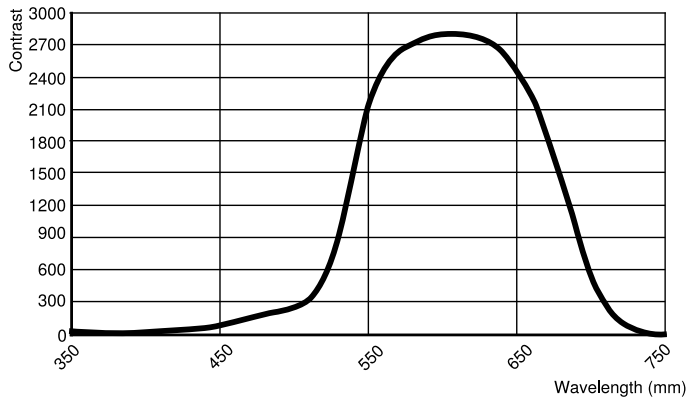
Transmission curve
