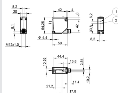
① Transmitter Diode ② Receiver Diode Screw M4 = 0.5 Nm
