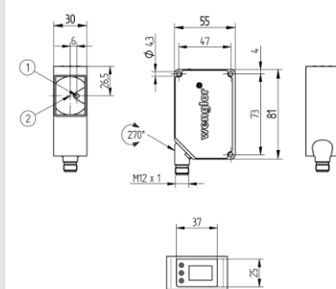
① Transmitter Diode ② Receiver Diode Screw M4 = 0.5 Nm
