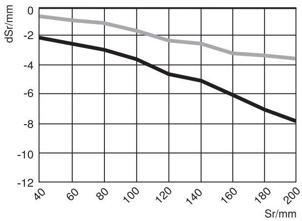
Illustration 1: Switching Distance Deviation P1MH
