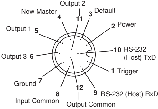
M12 12-Pin Plug
