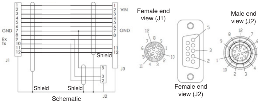
Schematic
