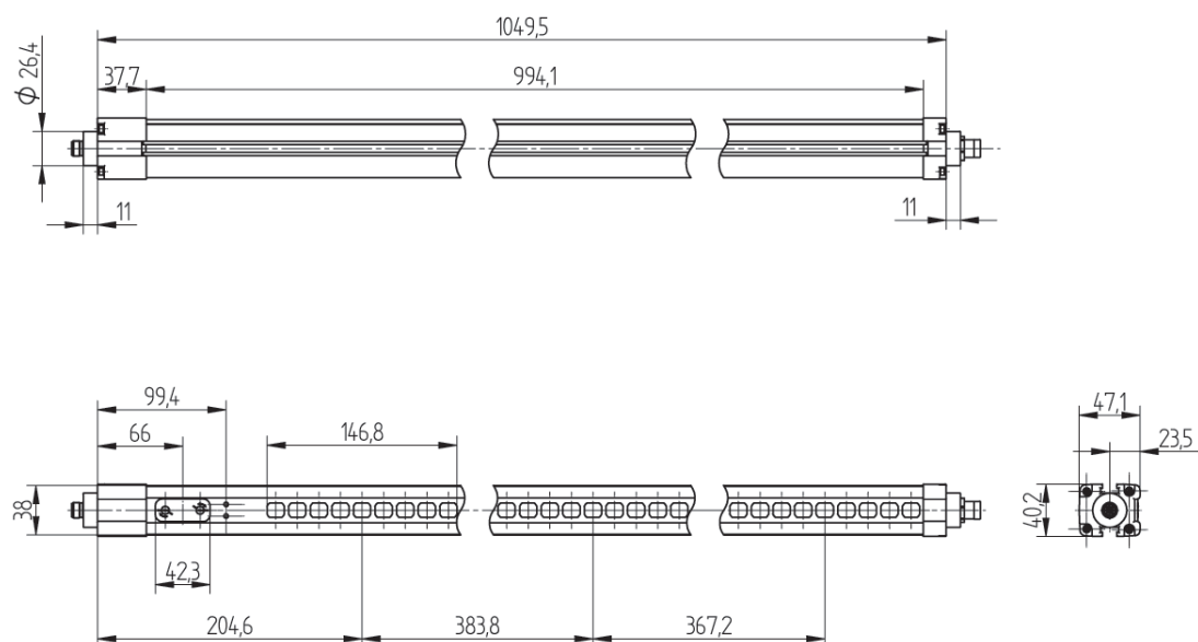
Emitter SB4-40IS080C1
