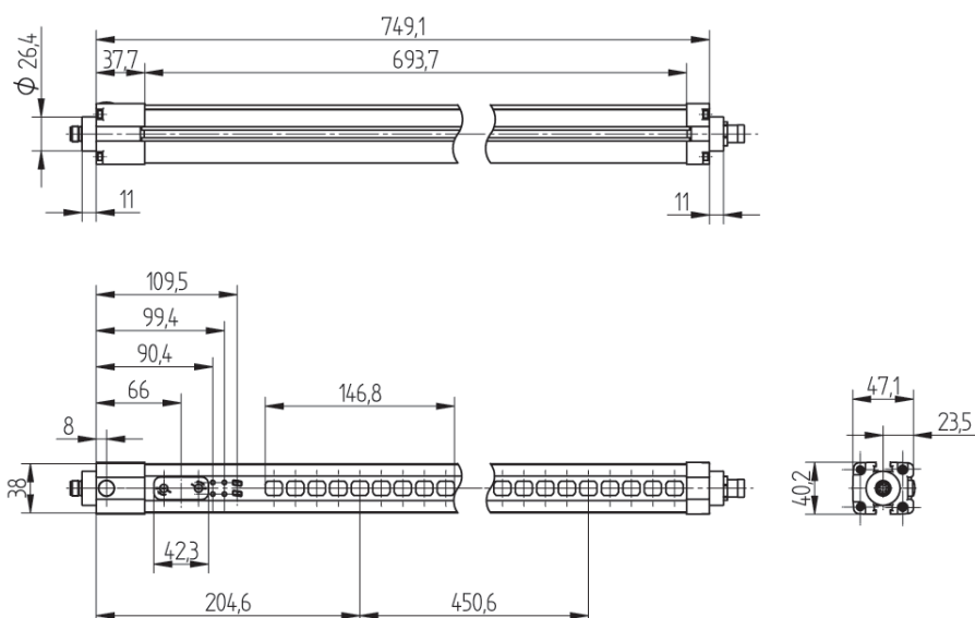
Receiver SB4-50IE050C1
