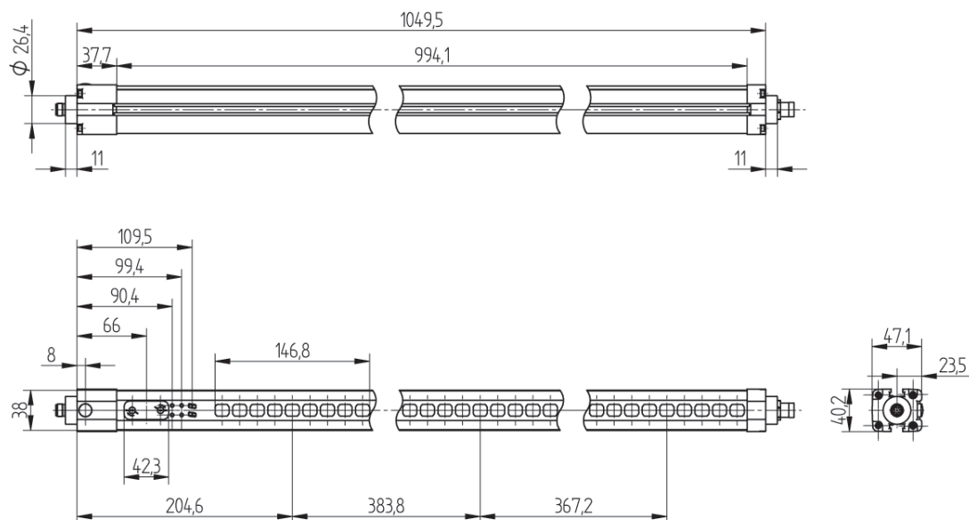
Receiver SB4-40IE080C1
