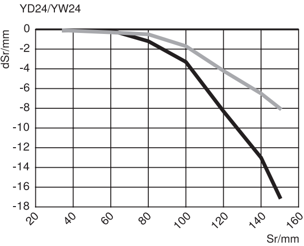
Illustration 1: Switching Distance Deviation
