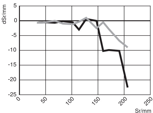
Illustration 1: Switching Distance Deviation OHD202A0103
