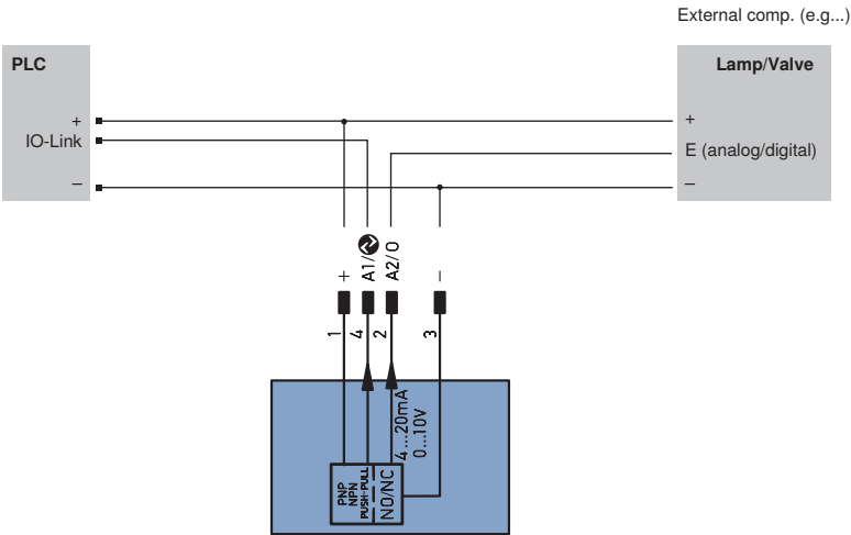
Figure 2: Wiring
