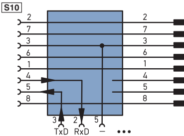
Connector cable M12×1, 8-pin (plug 2)
