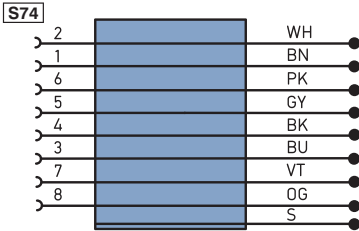
Interface cable (plug 1)
