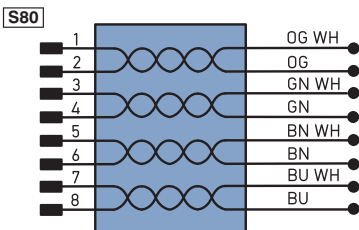
Connector cable M12×1, 8-pin (plug 2)
