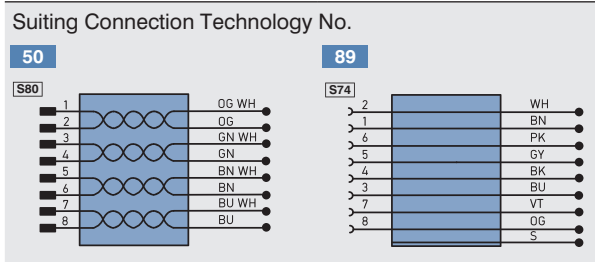
Connector cable M12×1, 8-pin (plug 1)
